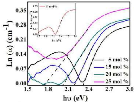
Figure 7 Plot of \ln(\alpha) vs. h\nu for the determination of Urbach energy.
