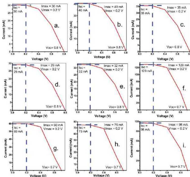
Figure 7. PV response of (a) TiO 2 , (b) Polyaniline(PANi), (c) Polythiophene (PTh), (d) Polypyrrole (PPy), (e) Polyindole (PIIn), (f) TiO 2 -Polyaniline composite (Ti-PANi), (g) TiO 2 -Polythiophene composite (Ti-PTh), (h) TiO 2 -Polypyrrole composite (Ti-PPy) and (i) TiO 2 -Polyindole composite (Ti-PIIn).
