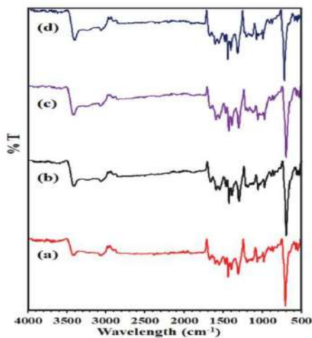
Figure 5. FTIR spectra of (a) PG1, (b) PG2, (c) PG3 and (d) PG4 composites.
