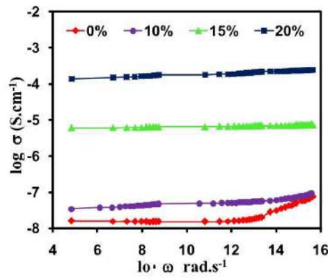
Fig. 6. Variation of Conductivity with mol % of Na 2 O 2 in temperature range 308–473 K.
