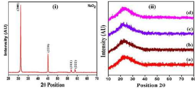
Fig. 1. (i) XRD of Sodium Superoxide ( \text{NaO}_2 ) and (ii) XRD of 60\text{V}_2\text{O}_5-5\text{P}_2\text{O}_5-(35-x)\text{B}_2\text{O}_7-x\text{NaO}_2 for (a) 0 mol%, (b) 10 mol%, (c) 15 mol% and (d) 20 mol% of \text{NaO}_2 .
