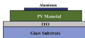
Fig. 1. Side face of fabricated PV cell.
