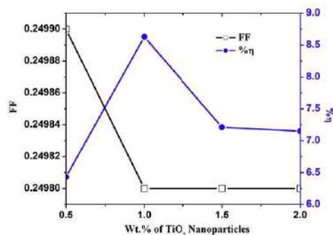
Fig. 13. Variation of FF and \% \eta as a function wt.% of \text{TiO}_2 nanoparticles in composites.
