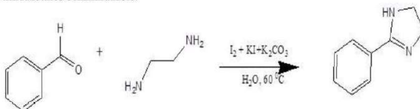
Figure 1 : Synthetic scheme of ligand
