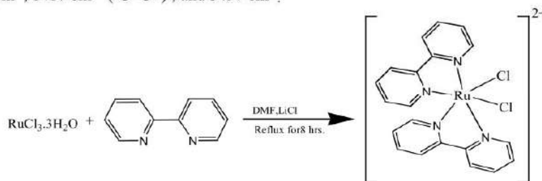
Figure 2: Synthetic scheme of P1
