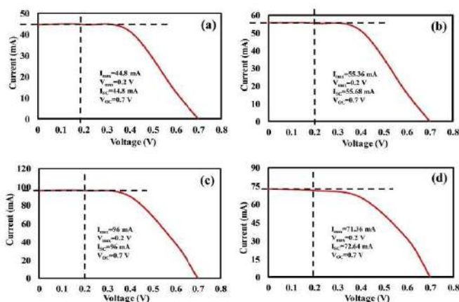
Fig. 6. PV response of (a) 5 wt%, (b) 10 wt%, (c) 15 wt% and (d) 20 wt% PANI loaded graphene composite.
