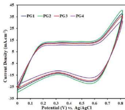
Figure 7. CV curves of PG1, PG2, PG3 and PG4 composites.
